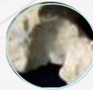
Anorthite
