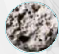
Porous Basalt
