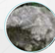
Bioclastic Limestone
