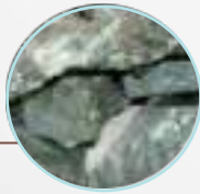
Serpentine
