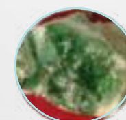
Volcanic Glass
