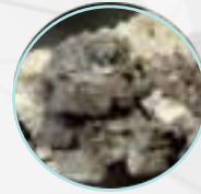
Zinc Spinel
