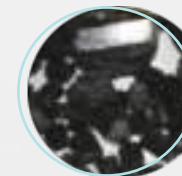
Tourmaline
